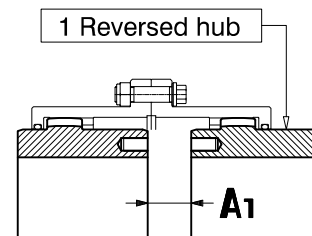
Fig. 02 - GO-AR Coupling
